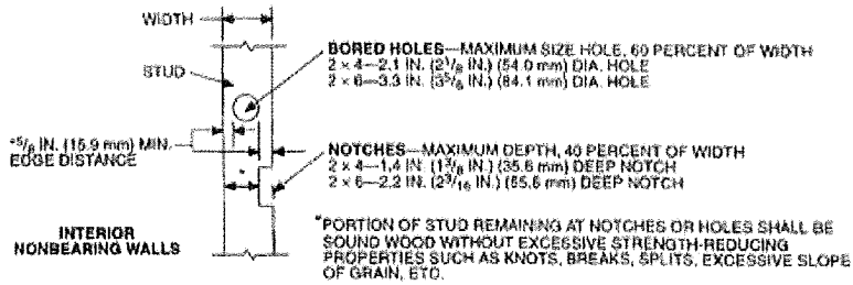
CUTTING, NOTCHING AND BORING OF STUDS
