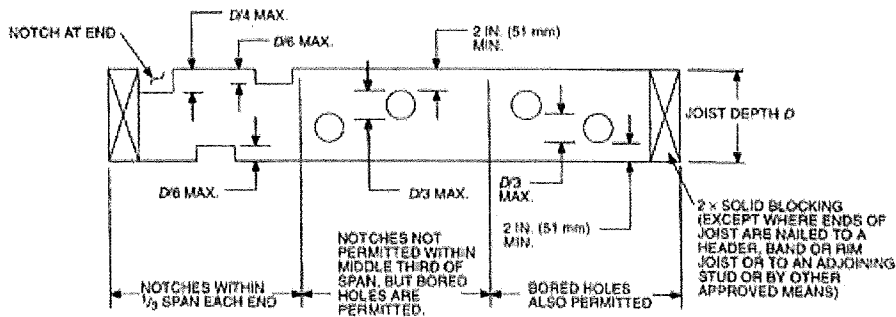
CUTTING, NOTCHING AND BORING OF FLOOR JOISTS
